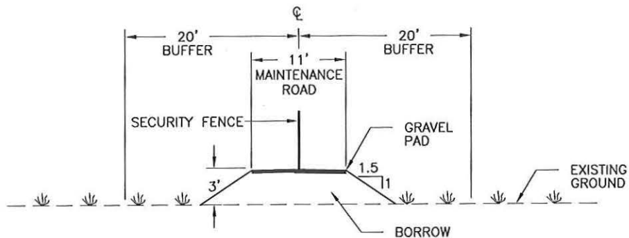
1 MAINTENANCE ROAD FOR FENCE - TYPICAL NOT TO SCALE
