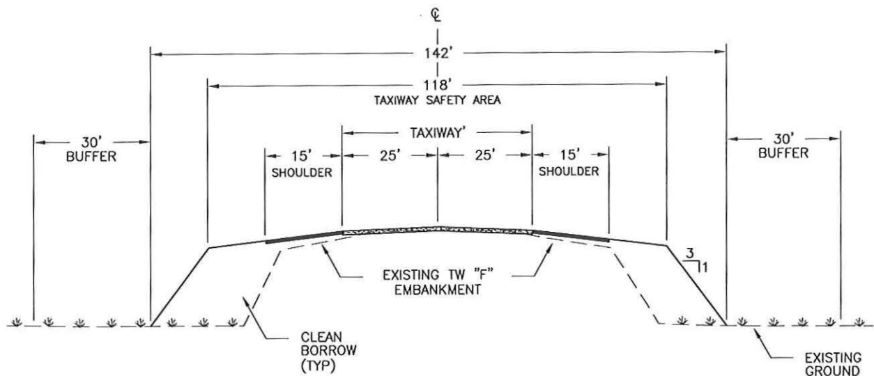
2 TAXIWAY (TW) F WIDENED EMBANKMENT - CROSS SECTION NOT TO SCALE
